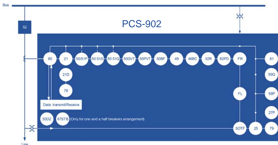
Figure 1 PCS-902 Functional Block Diagram
